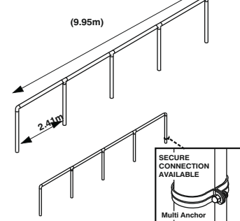
This is a Spectator Barrier that we supplied and Installed. 2.4m Rail with 1.5m socketed Post (0.5m underground)
